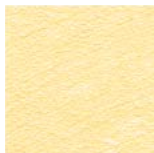
PYRITE
